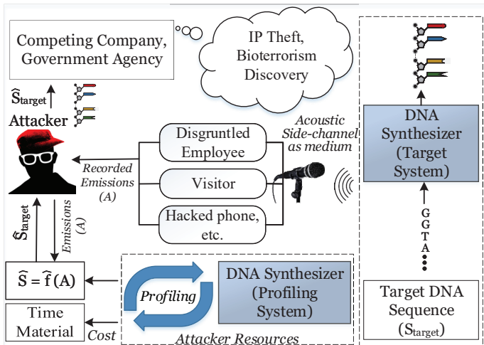
Fig. 4: Attack model.
