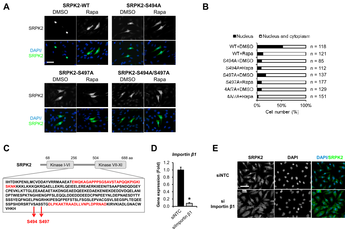
Figure S1. Further Characterization of SRPK2 Nuclear Localization, Related to Figure 3
