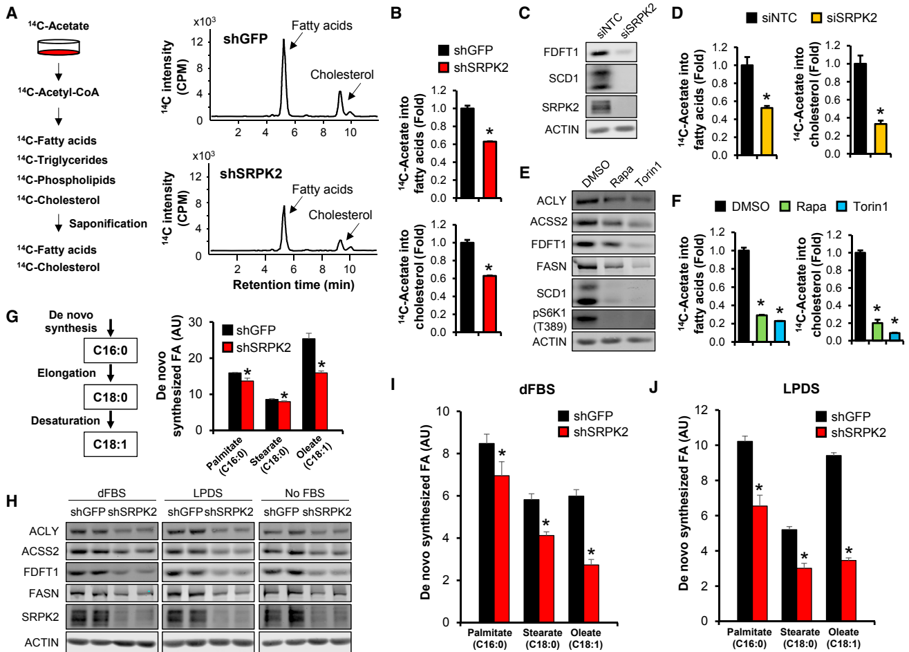
Figure 6. SRPK2 Is Necessary for De Novo Fatty Acid and Cholesterol Synthesis
