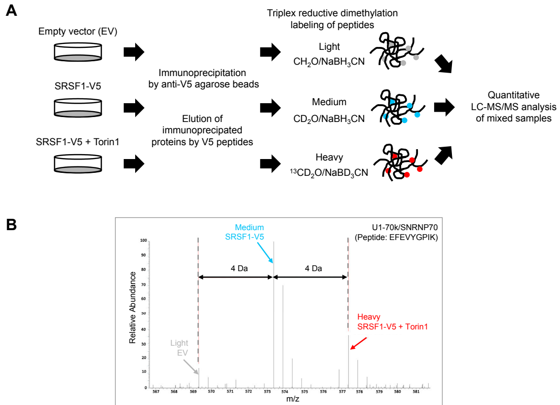
Figure S4. Interactome Analysis of SRSF1, Related to Figure 5
