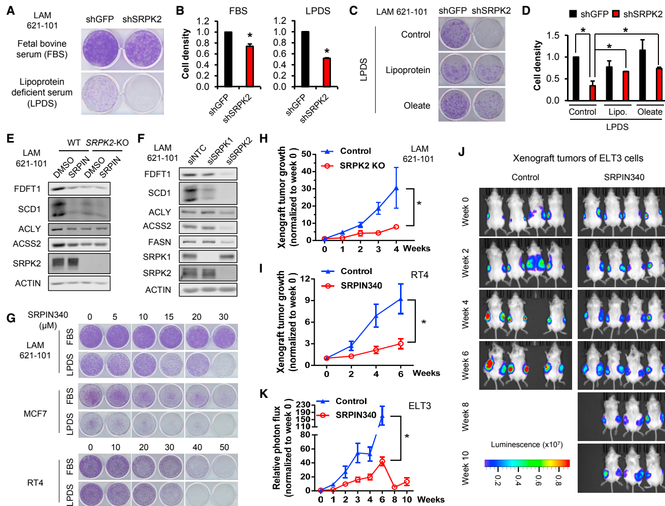
Figure 7. Inhibition of SRPK2 Blunts Cell Growth upon Lipid Starvation
