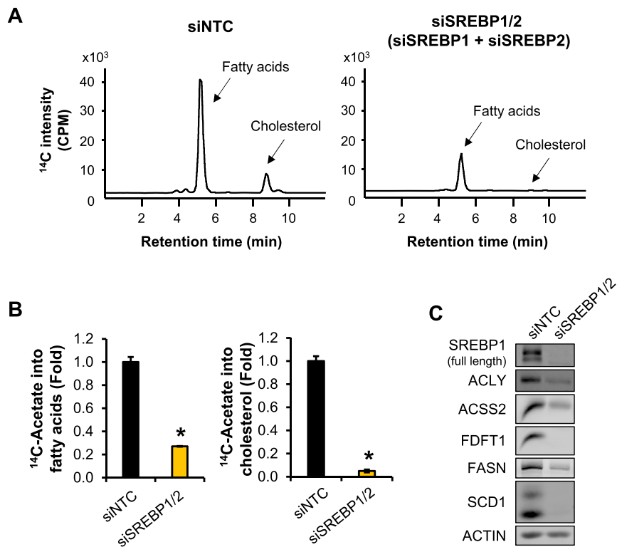
Figure S5. Further Characterization of Regulation of De Novo Lipogenesis by SREBP, Related to Figure 6
