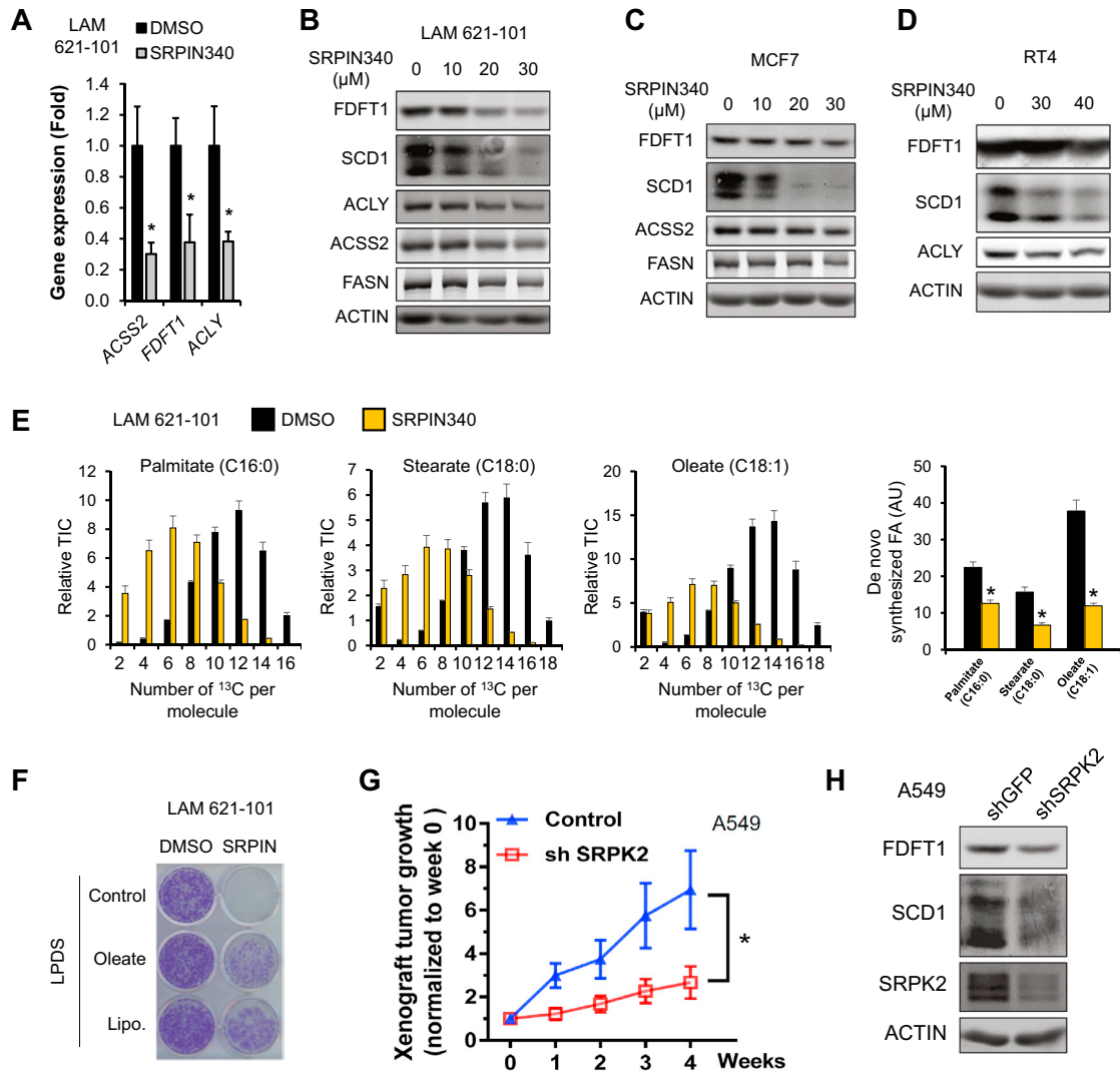
Figure S6. Further Characterization of SRPIN340, Related to Figure 7
