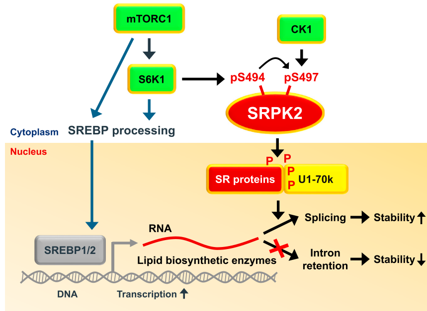
Figure S7. Proposed Model for the Regulation of Lipid Metabolism by mTORC1-SRPK2 Signaling Pathway, Related to Figure 7
